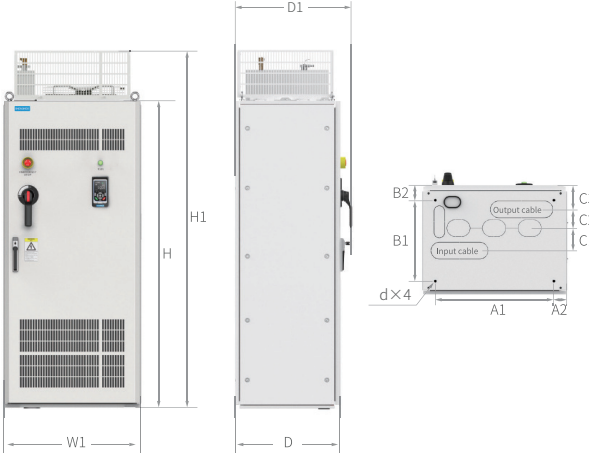
T13 (Without Auxiliary Power Distribution Cabinets)
