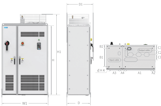
T13 (With Auxiliary Power Distribution Cabinets)
